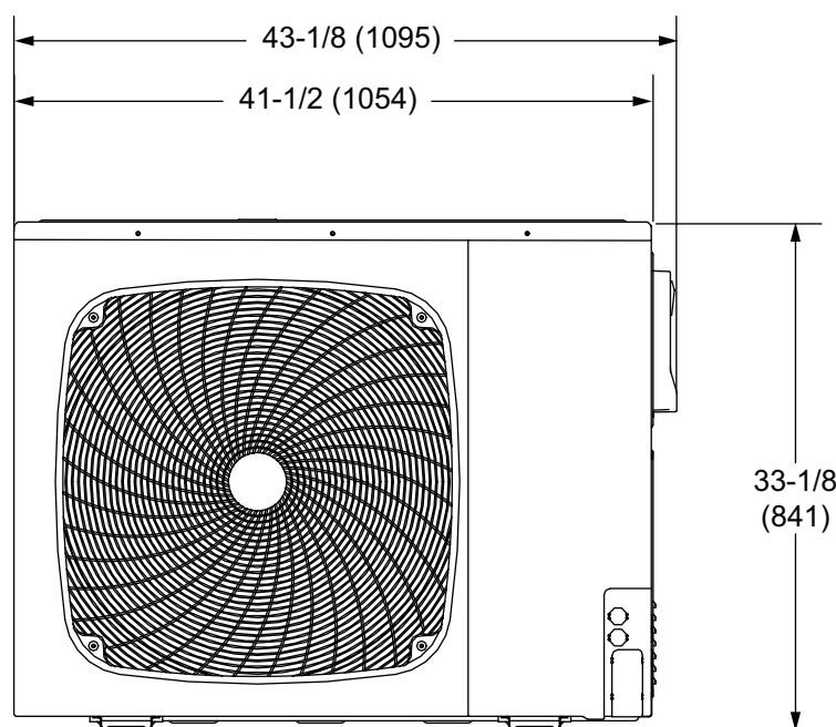
FRONT VIEW
